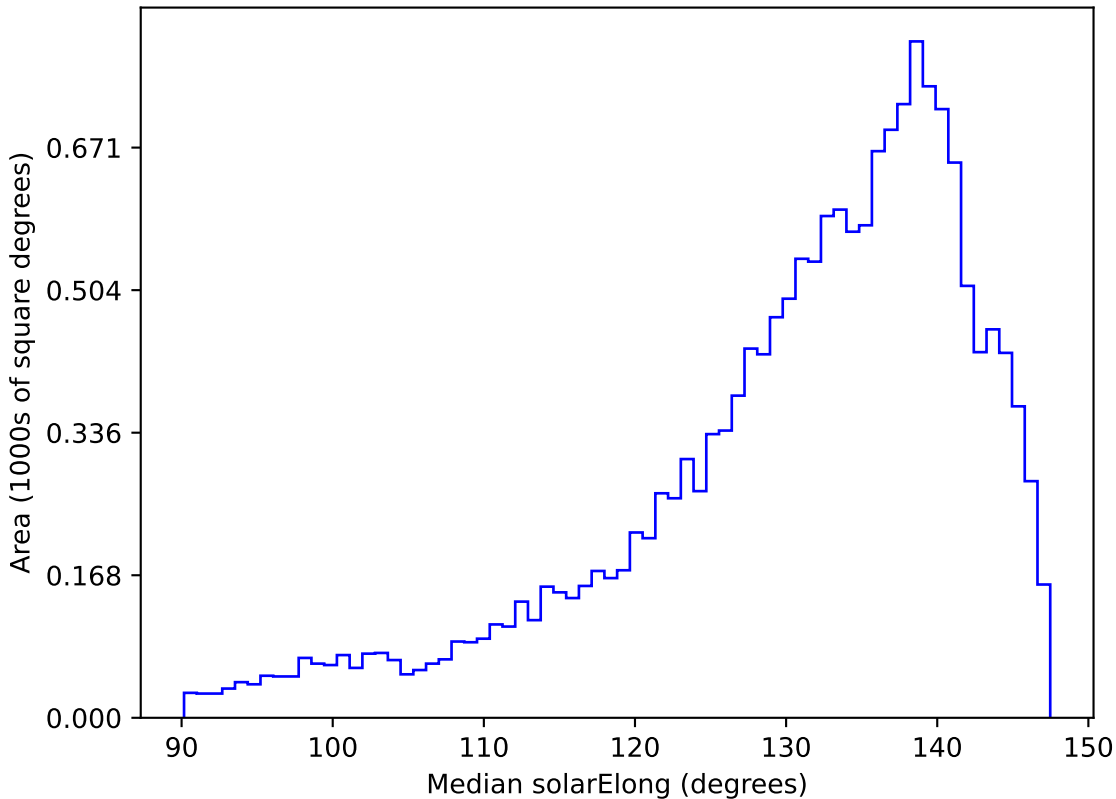
too_elab_r8_d2_griz_v3.4_10yrs WFD r band: Median solarElong
