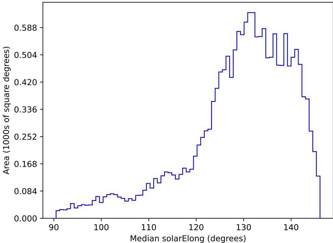
too_elab_r8_d2_griz_v3.4_10yrs WFD i band: Median solarElong
