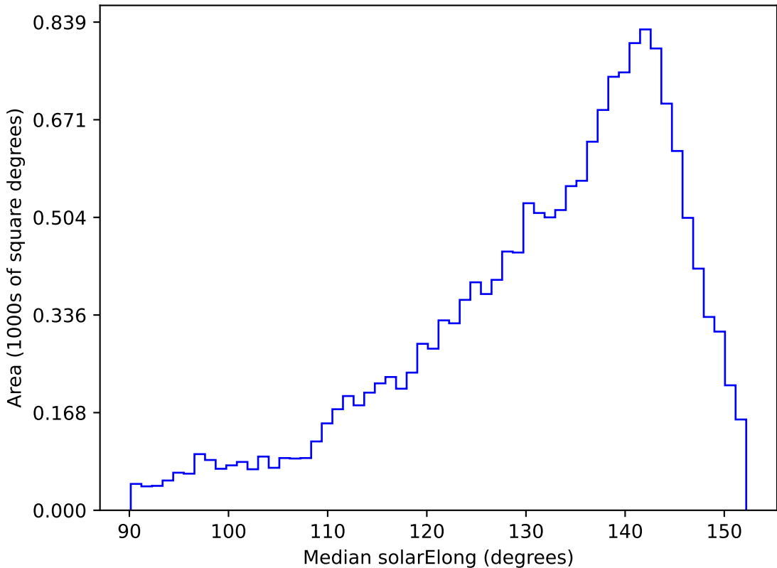
too_elab_r8_d2_griz_v3.4_10yrs WFD g band: Median solarElong
