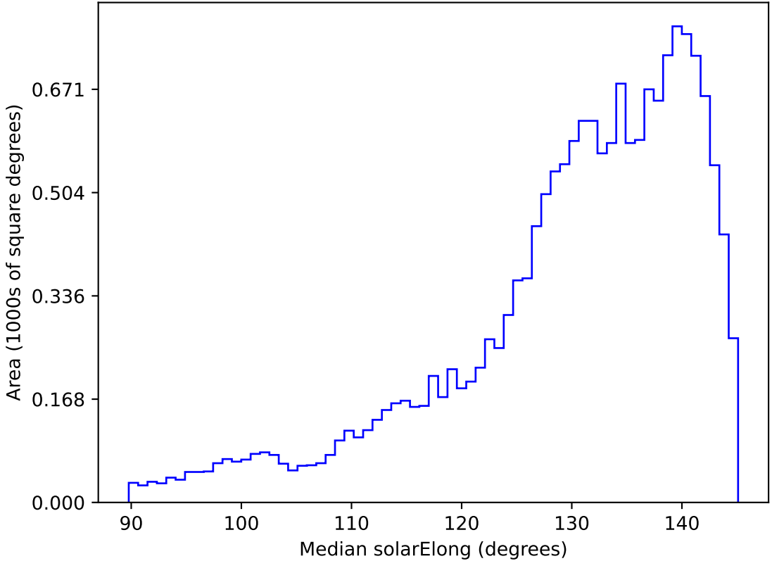
too_elab_r8_d2_griz_v3.4_10yrs WFD all bands: Median solarElong
