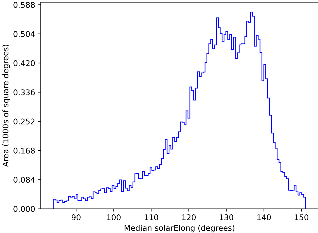
too_elab_r8_d2_griz_v3.4_10yrs All sky z band: Median solarElong
