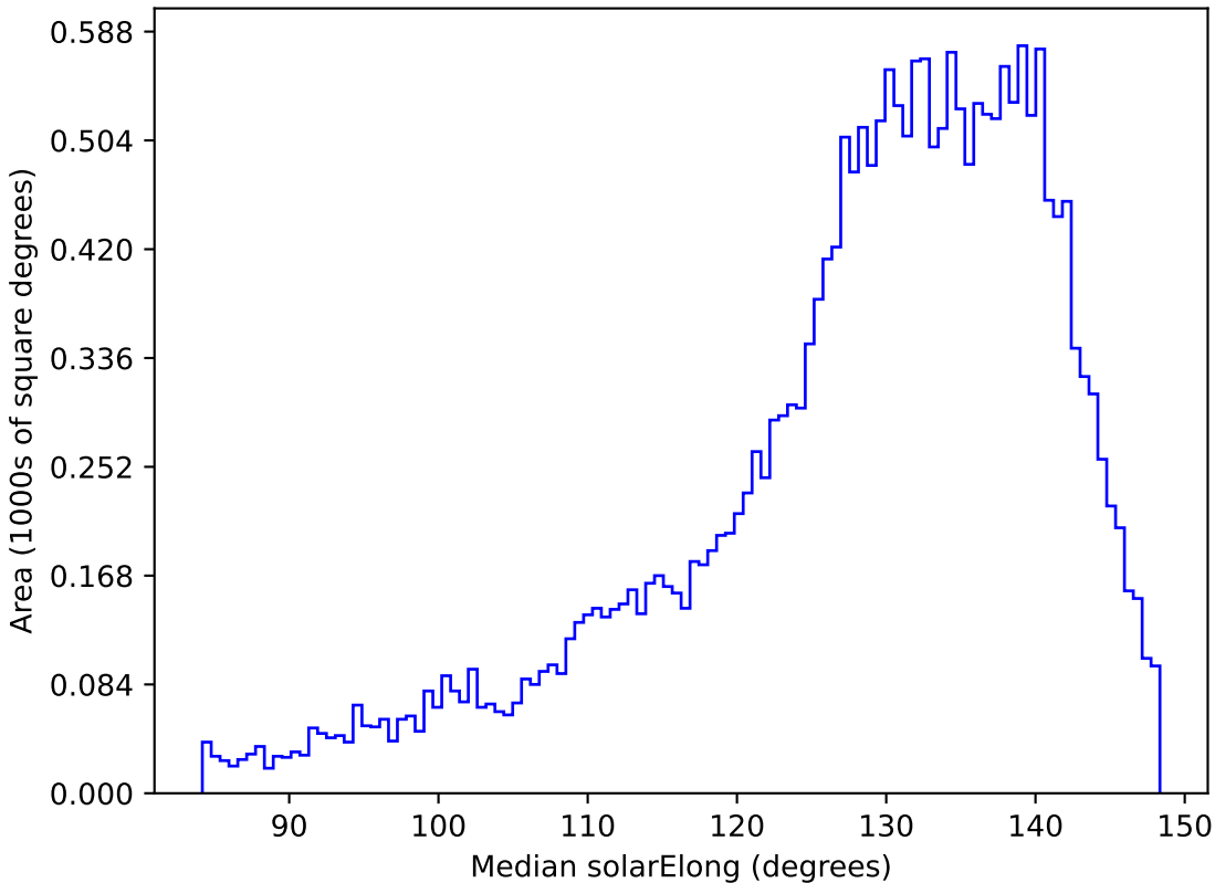
too_elab_r8_d2_griz_v3.4_10yrs All sky y band: Median solarElong
