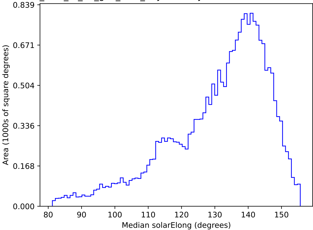
too_elab_r8_d2_griz_v3.4_10yrs All sky u band: Median solarElong
