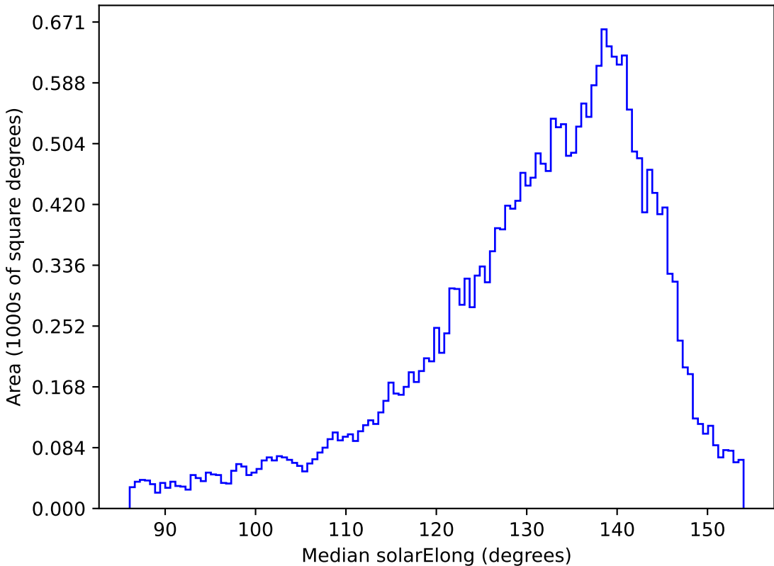
too_elab_r8_d2_griz_v3.4_10yrs All sky r band: Median solarElong
