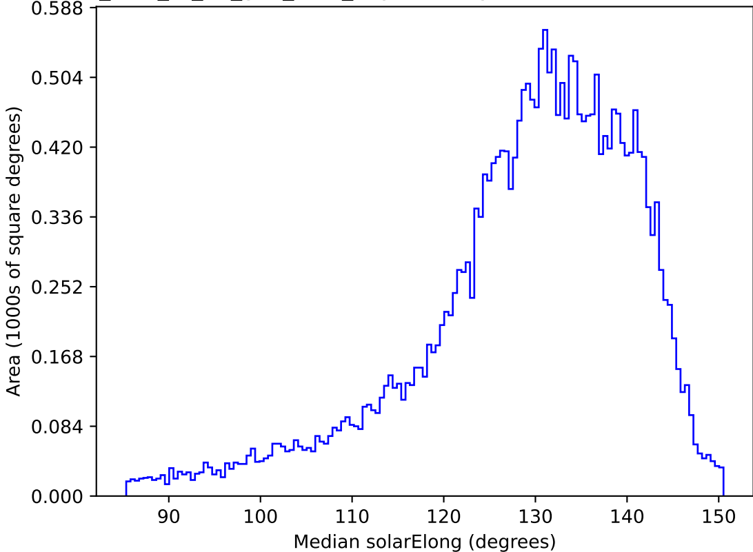
too_elab_r8_d2_griz_v3.4_10yrs All sky i band: Median solarElong
