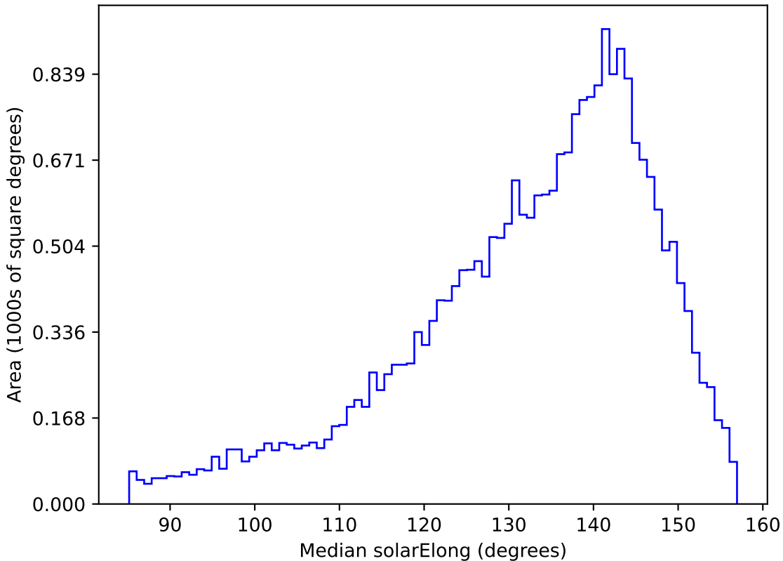
too_elab_r8_d2_griz_v3.4_10yrs All sky g band: Median solarElong
