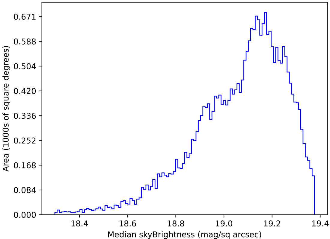
too_elab_r8_d2_griz_v3.4_10yrs Yr 1 z band: Median skyBrightness
