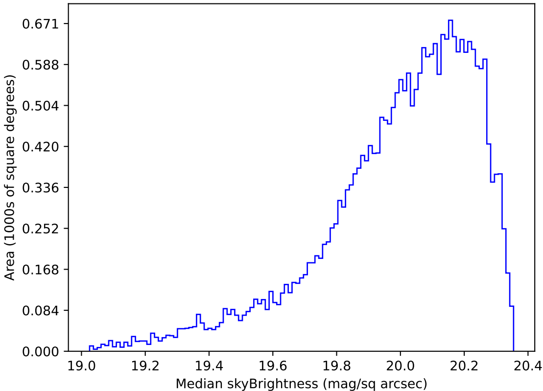
too_elab_r8_d2_griz_v3.4_10yrs Yr 1 i band: Median skyBrightness
