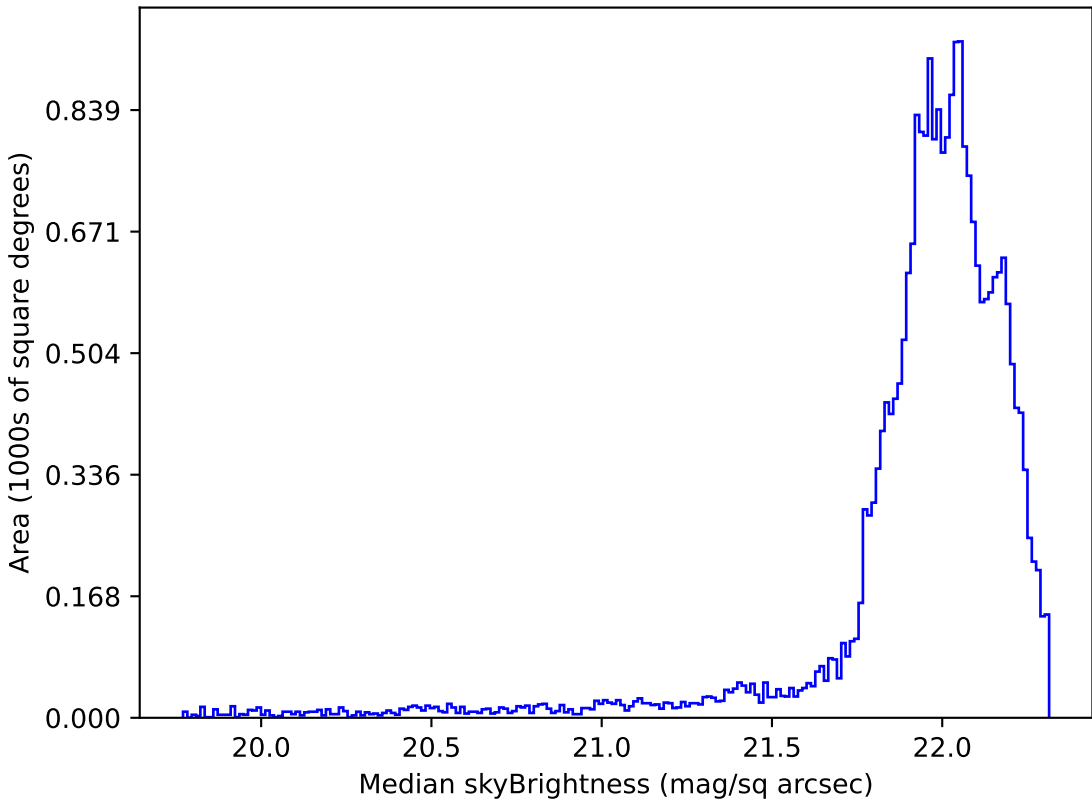
too_elab_r8_d2_griz_v3.4_10yrs Yr 1 g band: Median skyBrightness
