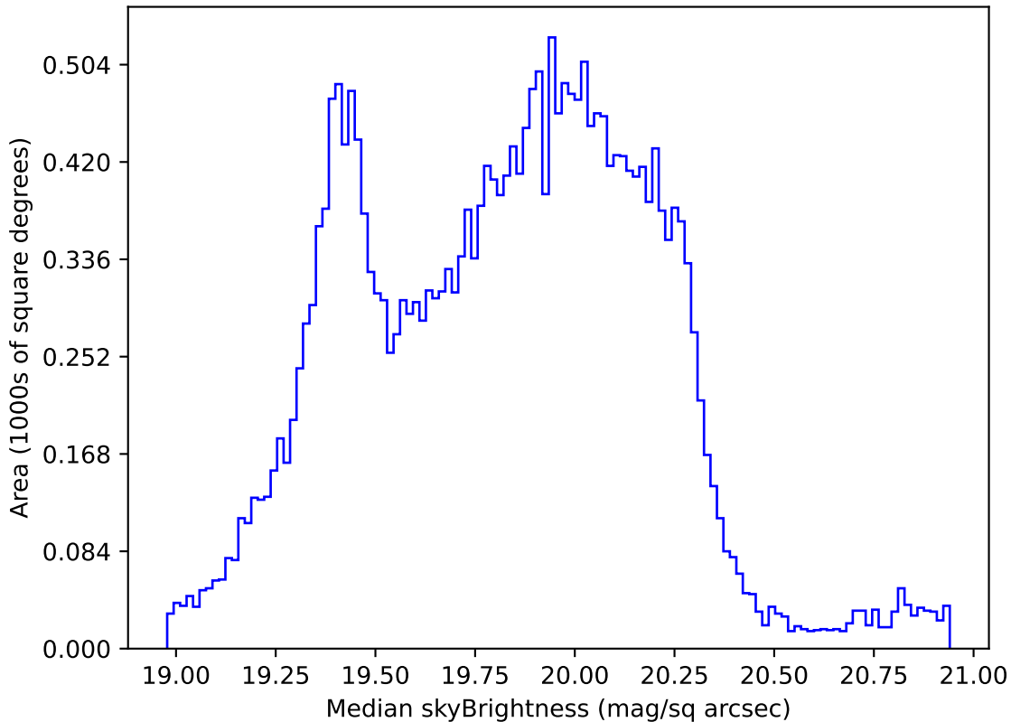
too_elab_r8_d2_griz_v3.4_10yrs Yr 1 all bands: Median skyBrightness
