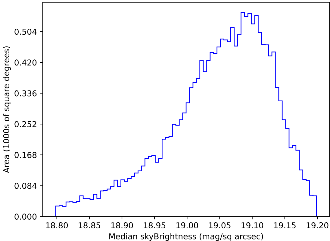
too_elab_r8_d2_griz_v3.4_10yrs WFD z band: Median skyBrightness
