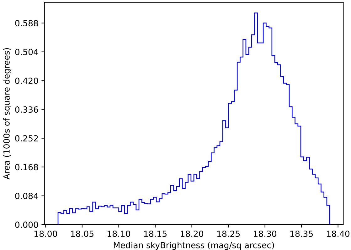
too_elab_r8_d2_griz_v3.4_10yrs WFD y band: Median skyBrightness
