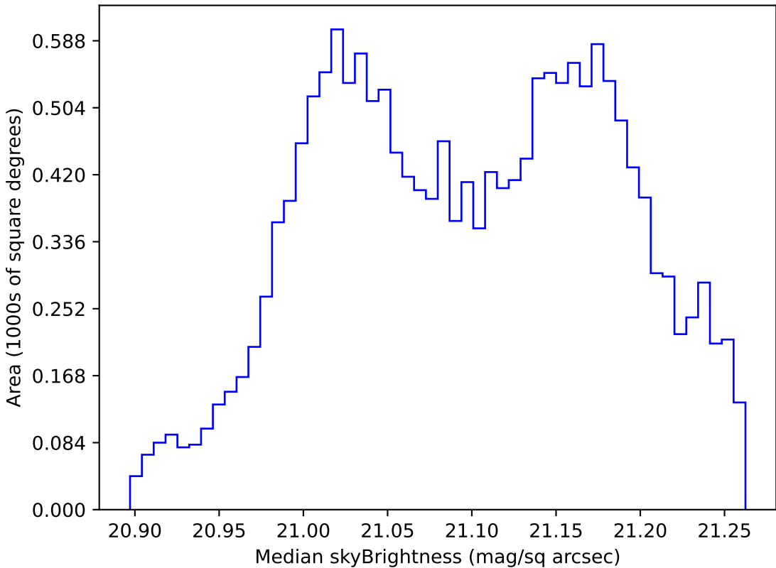
too_elab_r8_d2_griz_v3.4_10yrs WFD r band: Median skyBrightness
