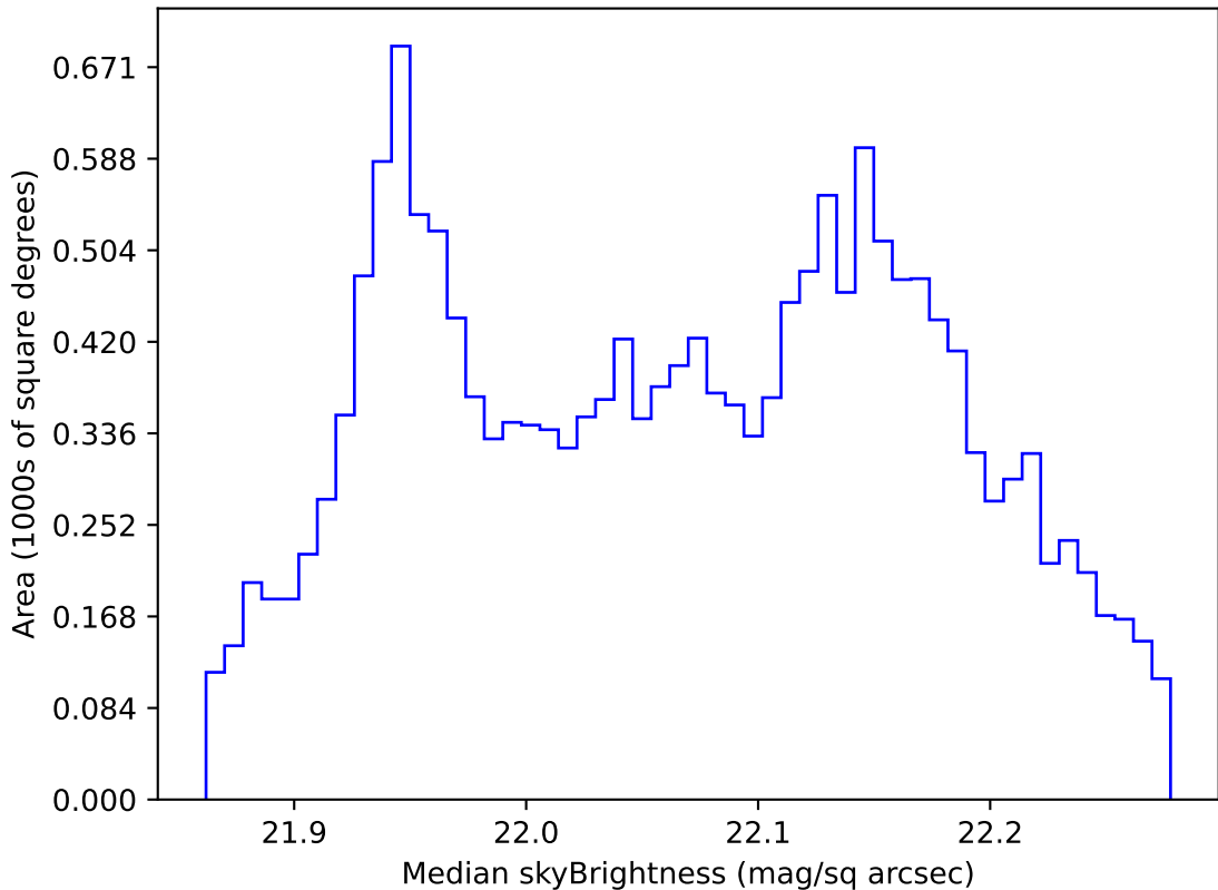
too_elab_r8_d2_griz_v3.4_10yrs WFD g band: Median skyBrightness
