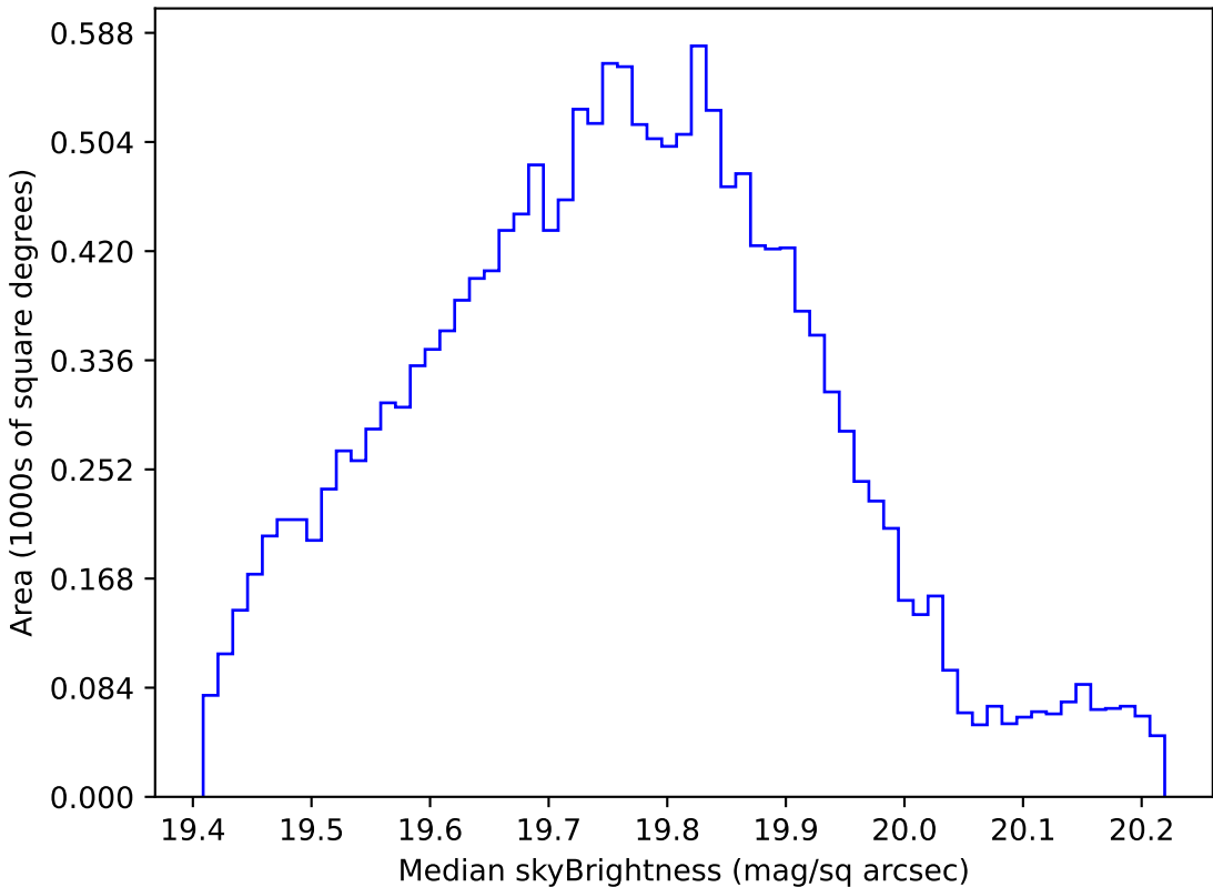
too_elab_r8_d2_griz_v3.4_10yrs WFD all bands: Median skyBrightness
