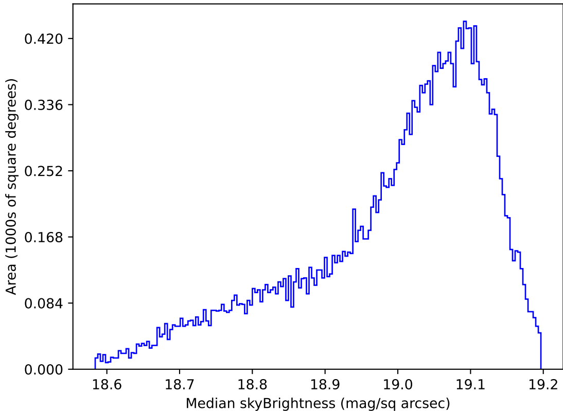
too_elab_r8_d2_griz_v3.4_10yrs All sky z band: Median skyBrightness
