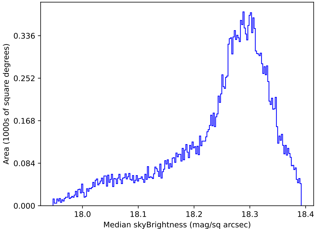
too_elab_r8_d2_griz_v3.4_10yrs All sky y band: Median skyBrightness
