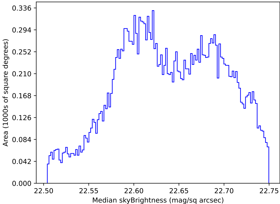
too_elab_r8_d2_griz_v3.4_10yrs All sky u band: Median skyBrightness
