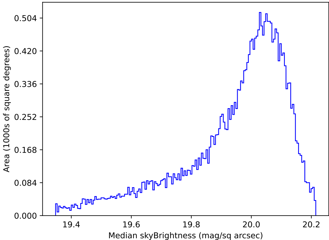
too_elab_r8_d2_griz_v3.4_10yrs All sky i band: Median skyBrightness
