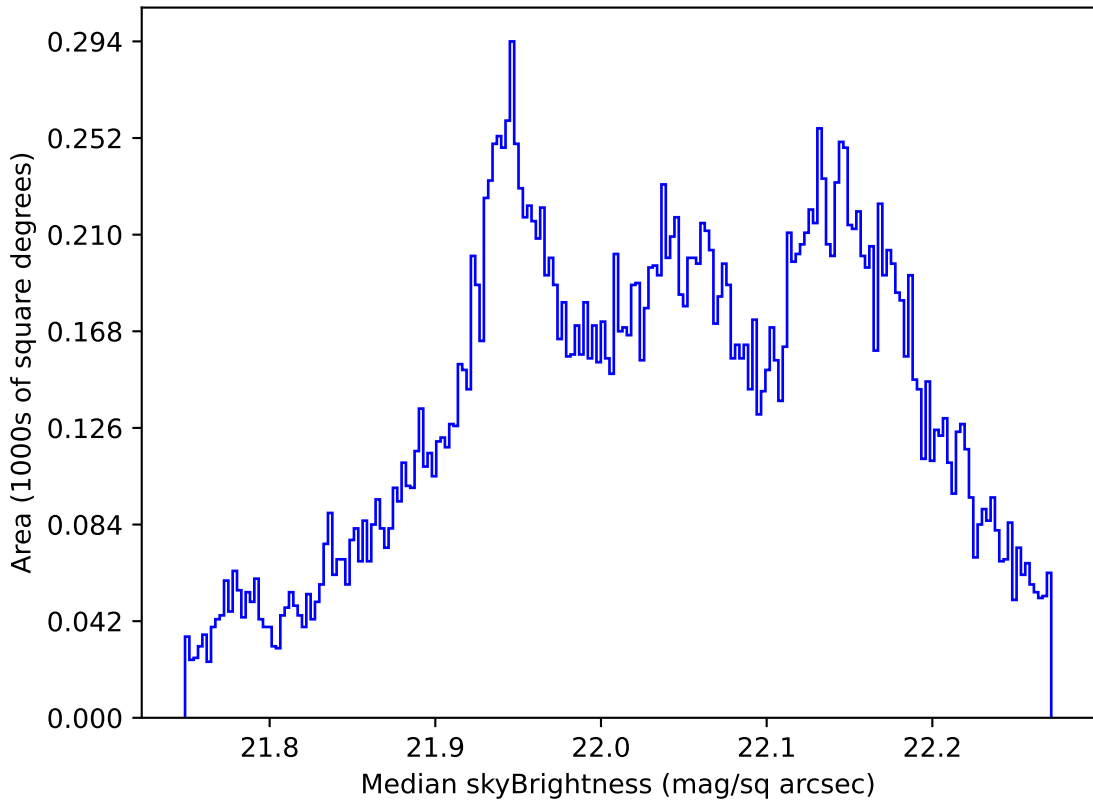
too_elab_r8_d2_griz_v3.4_10yrs All sky g band: Median skyBrightness
