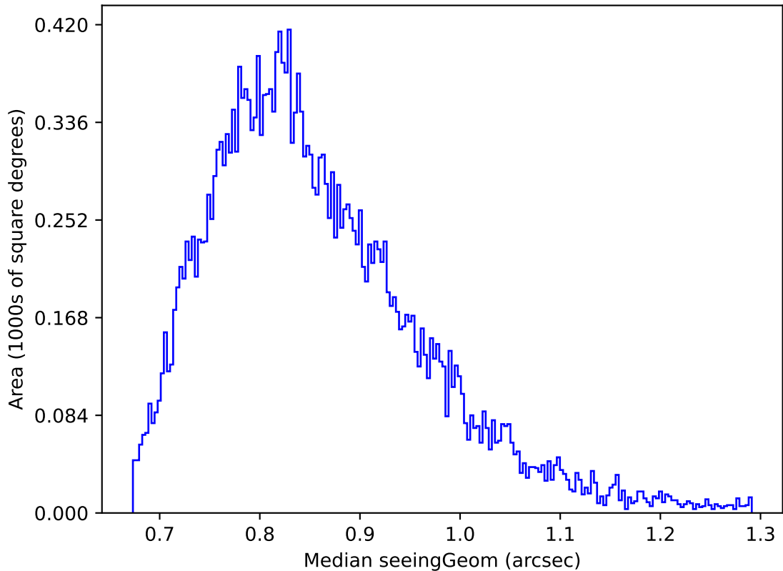
too_elab_r8_d2_griz_v3.4_10yrs Yr 1 z band: Median seeingGeom
