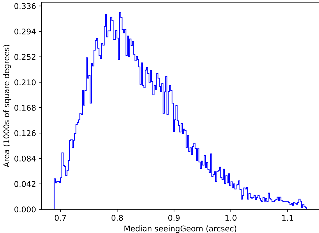
too_elab_r8_d2_griz_v3.4_10yrs Yr 1 y band: Median seeingGeom
