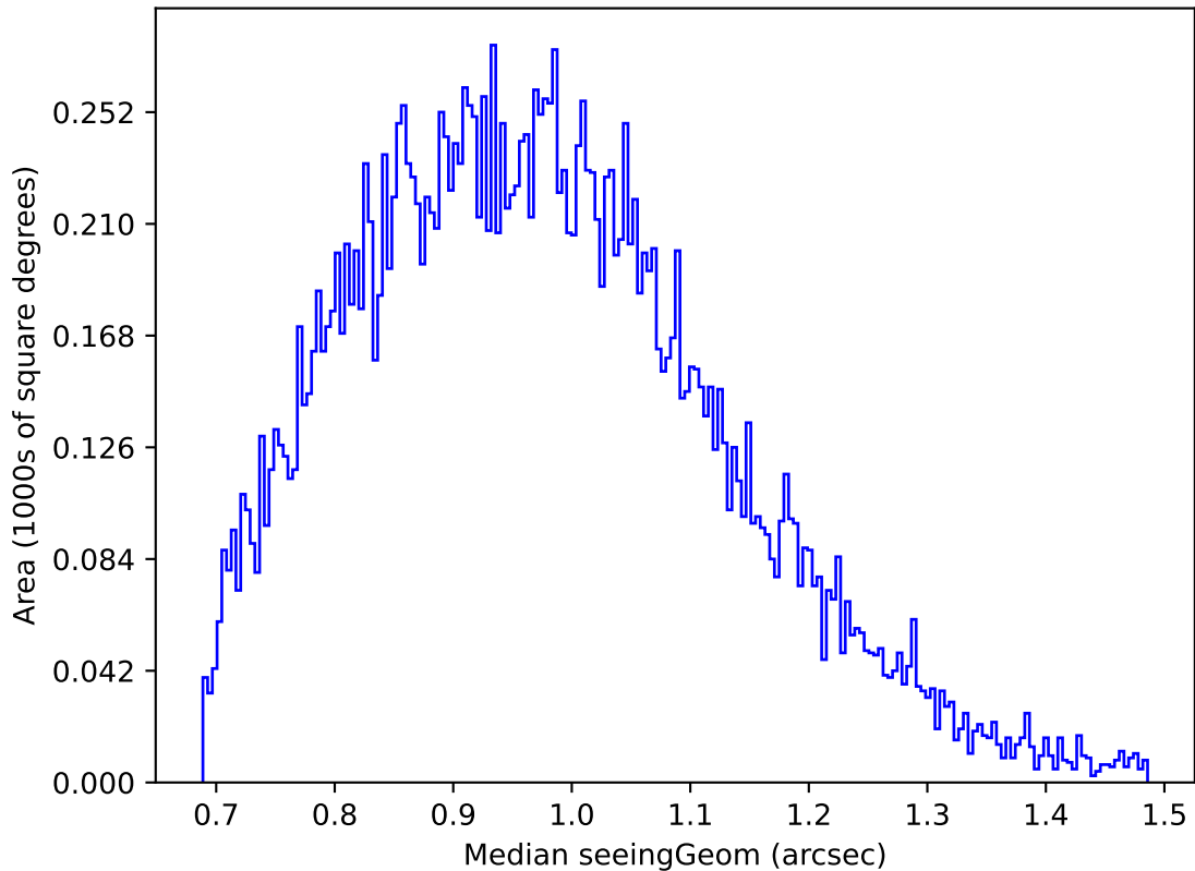
too_elab_r8_d2_griz_v3.4_10yrs Yr 1 u band: Median seeingGeom
