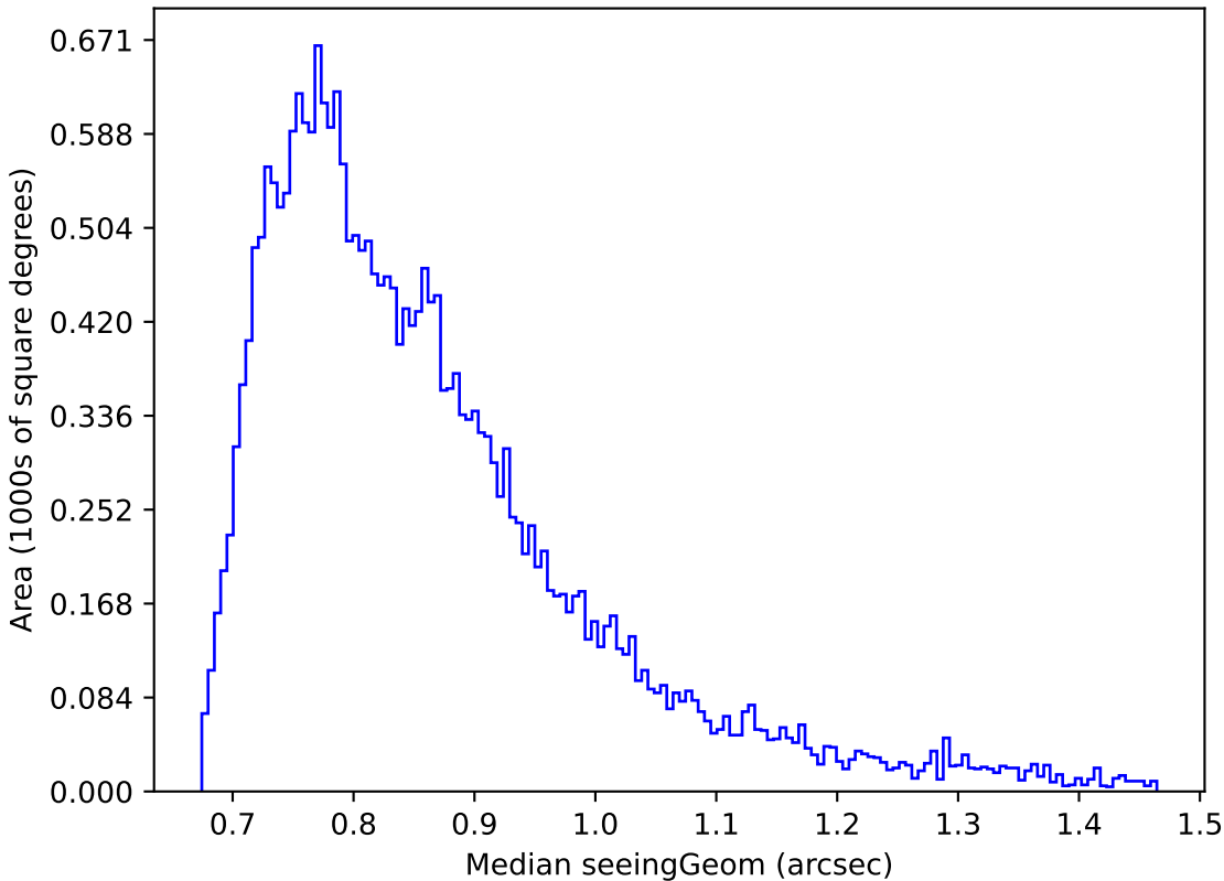
too_elab_r8_d2_griz_v3.4_10yrs Yr 1 r band: Median seeingGeom
