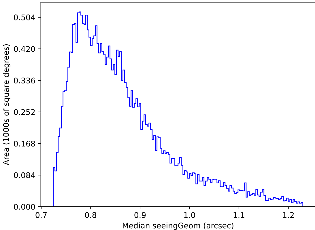
too_elab_r8_d2_griz_v3.4_10yrs Yr 1 all bands: Median seeingGeom
