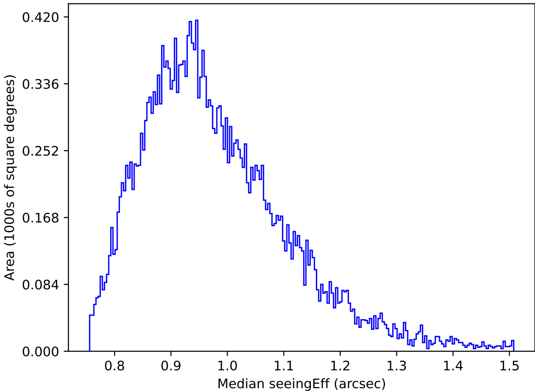
too_elab_r8_d2_griz_v3.4_10yrs Yr 1 z band: Median seeingEff
