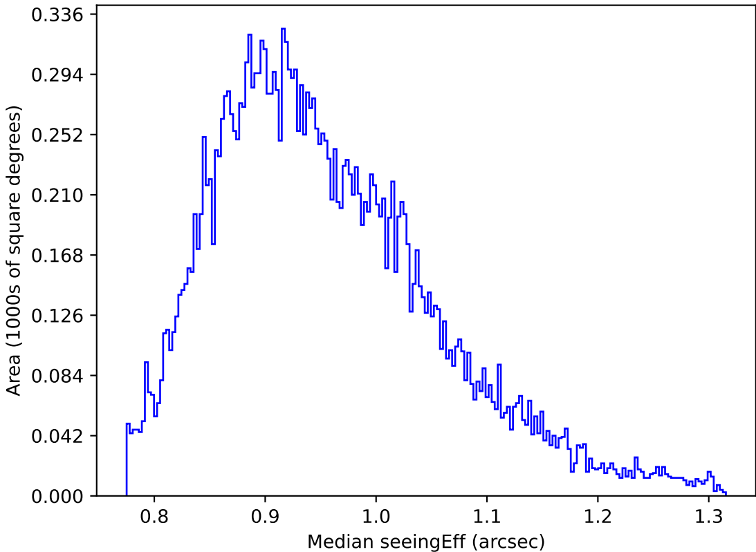
too_elab_r8_d2_griz_v3.4_10yrs Yr 1 y band: Median seeingEff
