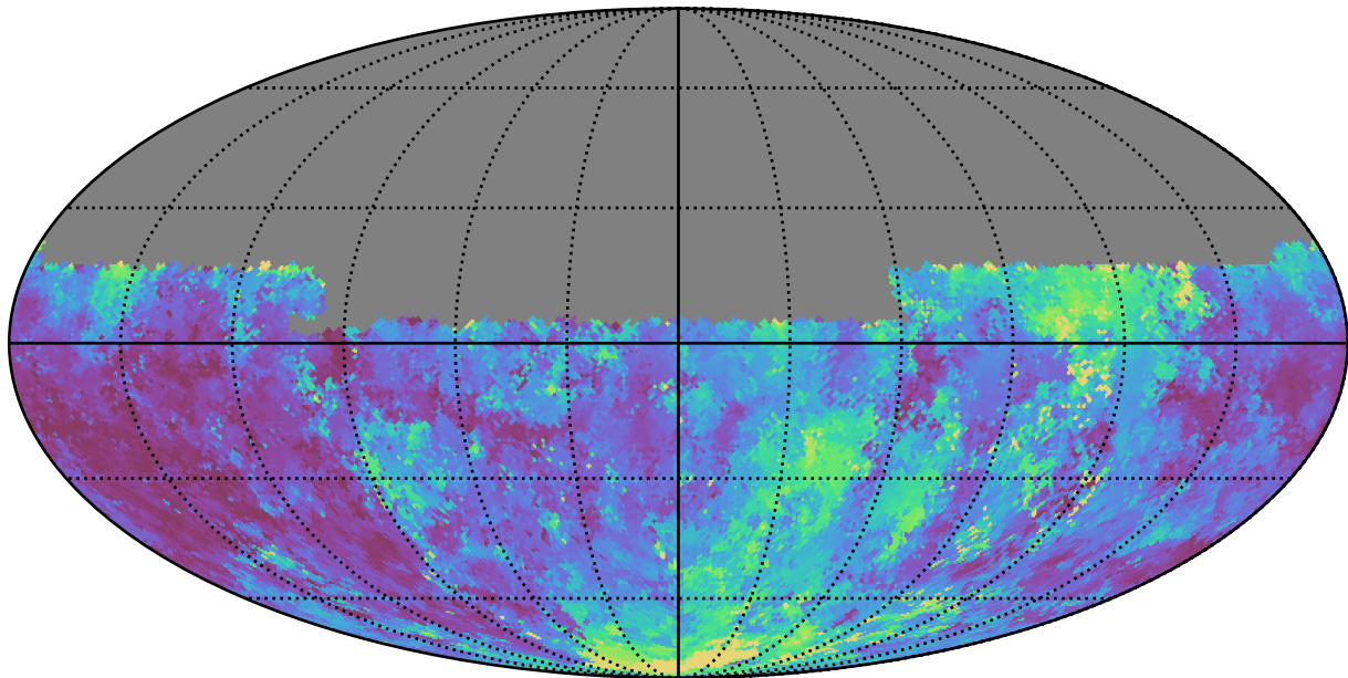
too_elab_r8_d2_griz_v3.4_10yrs Yr 1 u band: Median seeingEff
