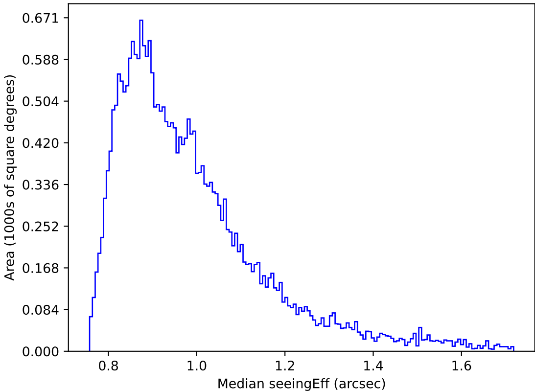
too_elab_r8_d2_griz_v3.4_10yrs Yr 1 r band: Median seeingEff
