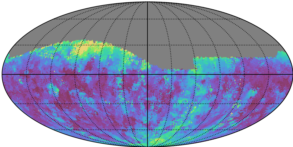
too_elab_r8_d2_griz_v3.4_10yrs Yr 1 g band: Median seeingEff
