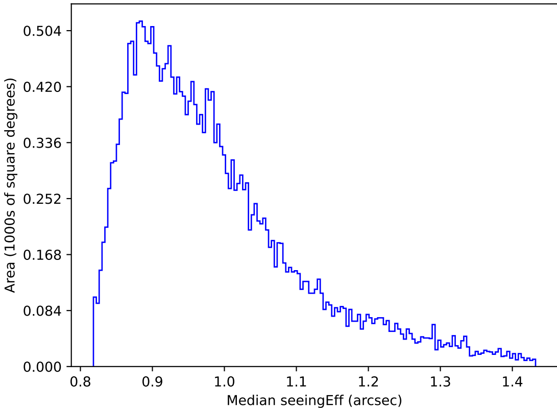
too_elab_r8_d2_griz_v3.4_10yrs Yr 1 all bands: Median seeingEff
