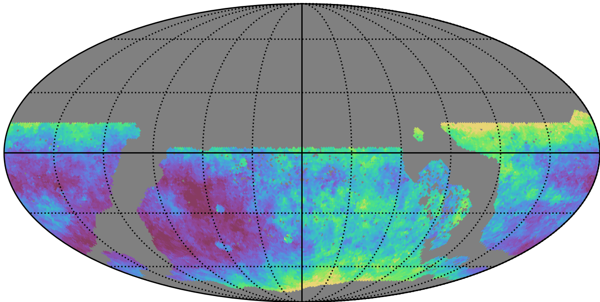
too_elab_r8_d2_griz_v3.4_10yrs WFD z band: Median seeingEff
