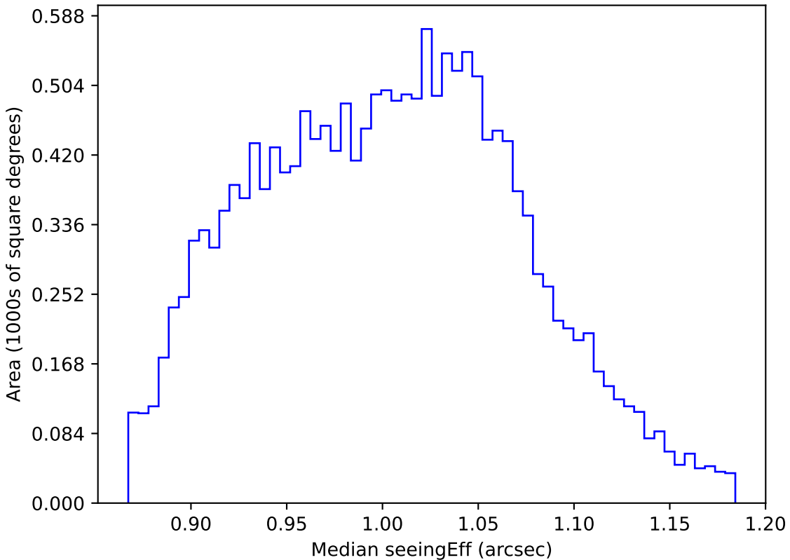
too_elab_r8_d2_griz_v3.4_10yrs WFD z band: Median seeingEff
