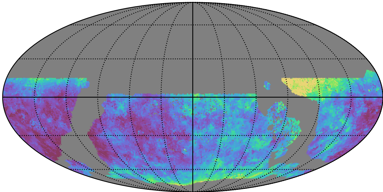
too_elab_r8_d2_griz_v3.4_10yrs WFD u band: Median seeingEff
