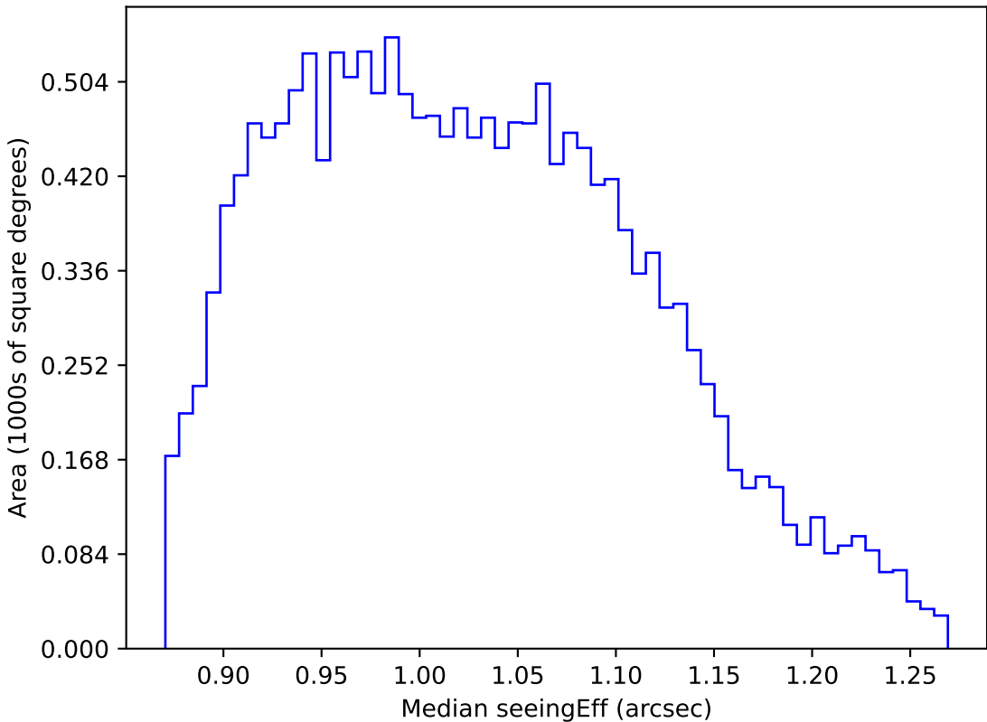
too_elab_r8_d2_griz_v3.4_10yrs WFD r band: Median seeingEff
