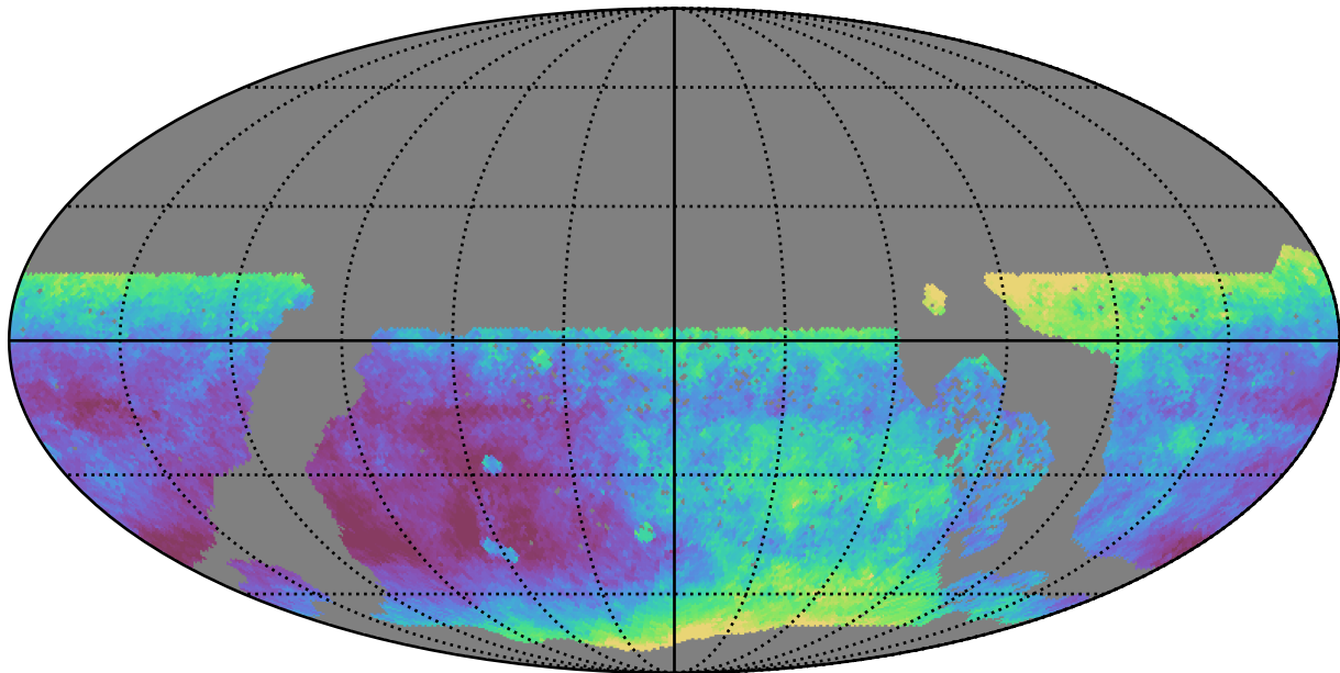
too_elab_r8_d2_griz_v3.4_10yrs WFD i band: Median seeingEff
