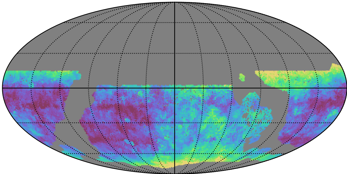
too_elab_r8_d2_griz_v3.4_10yrs WFD g band: Median seeingEff
