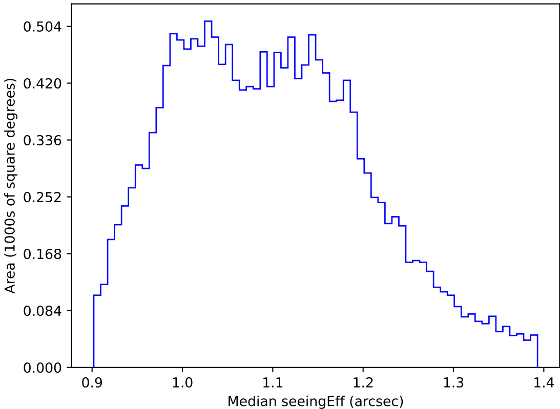
too_elab_r8_d2_griz_v3.4_10yrs WFD g band: Median seeingEff
