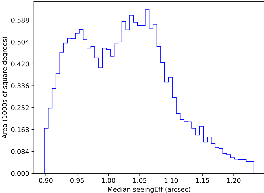
too_elab_r8_d2_griz_v3.4_10yrs WFD all bands: Median seeingEff
