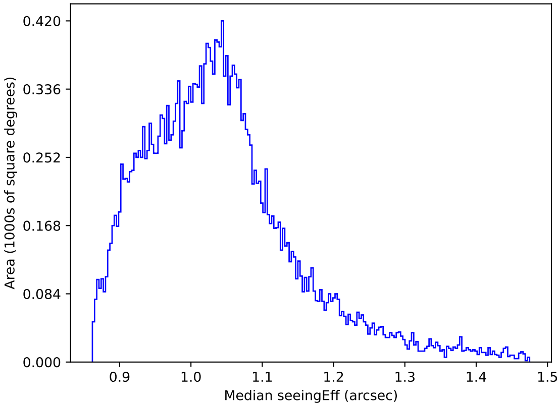
too_elab_r8_d2_griz_v3.4_10yrs All sky z band: Median seeingEff
