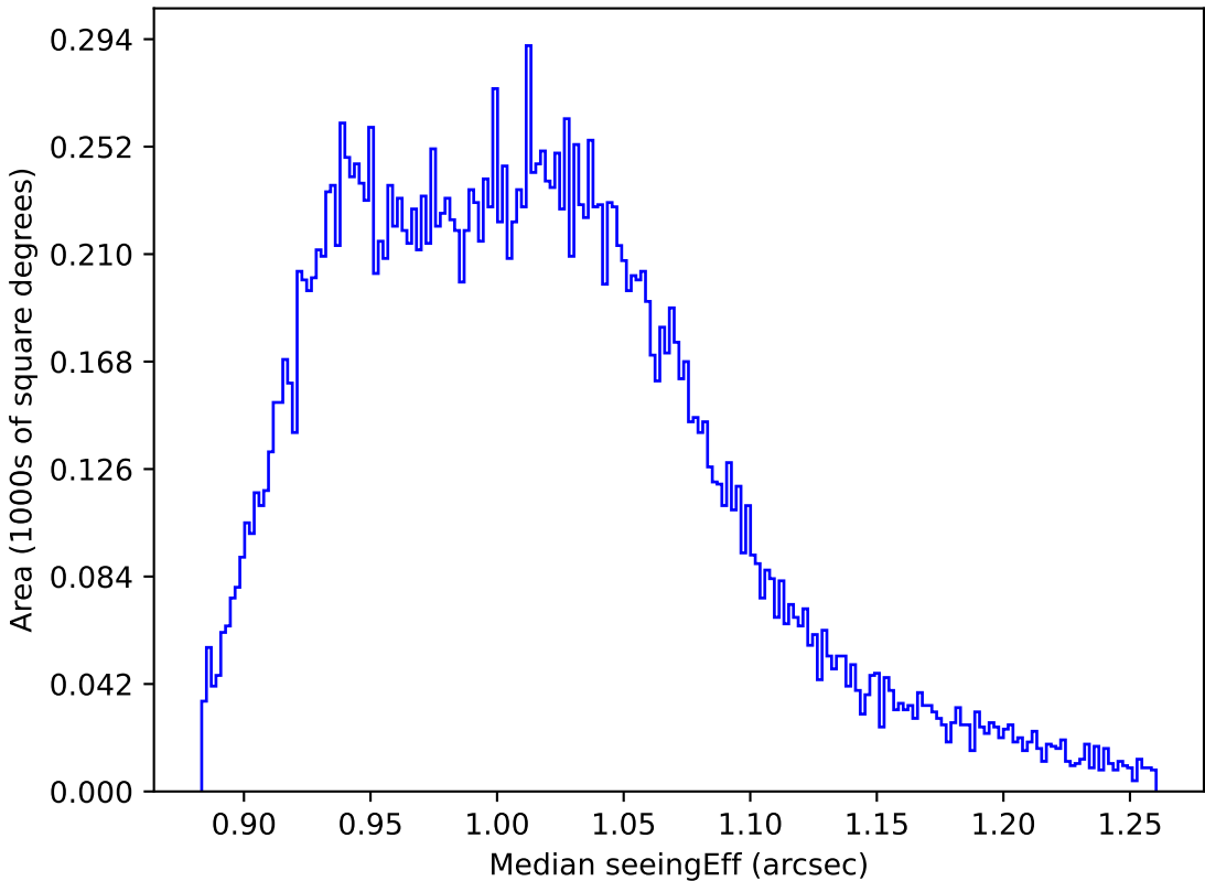
too_elab_r8_d2_griz_v3.4_10yrs All sky y band: Median seeingEff
