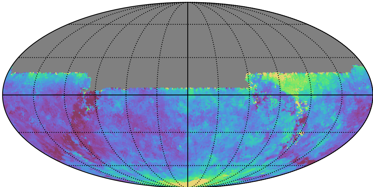
too_elab_r8_d2_griz_v3.4_10yrs All sky u band: Median seeingEff
