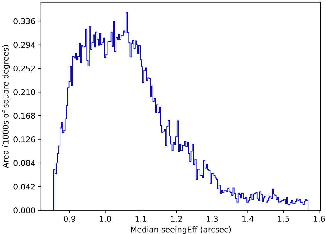
too_elab_r8_d2_griz_v3.4_10yrs All sky r band: Median seeingEff
