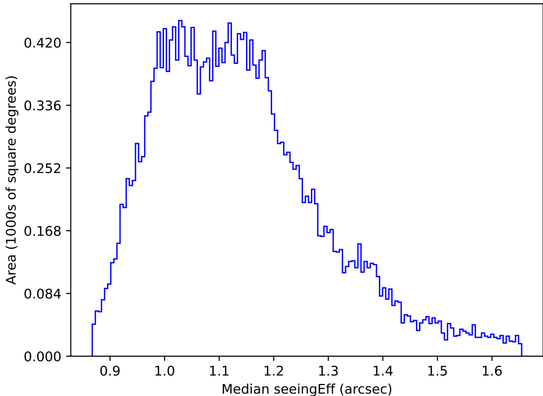
too_elab_r8_d2_griz_v3.4_10yrs All sky g band: Median seeingEff
