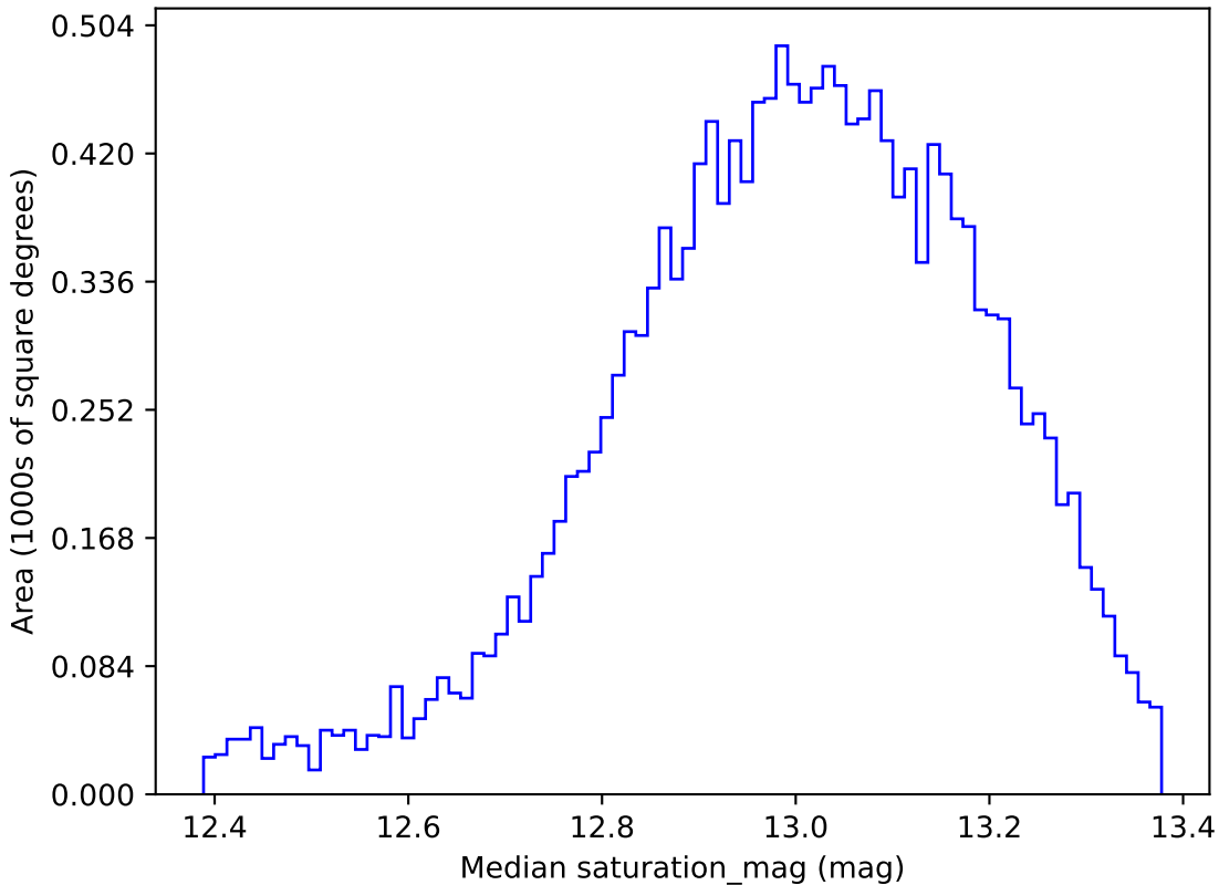
too_elab_r8_d2_griz_v3.4_10yrs WFD u band: Median saturation_mag
