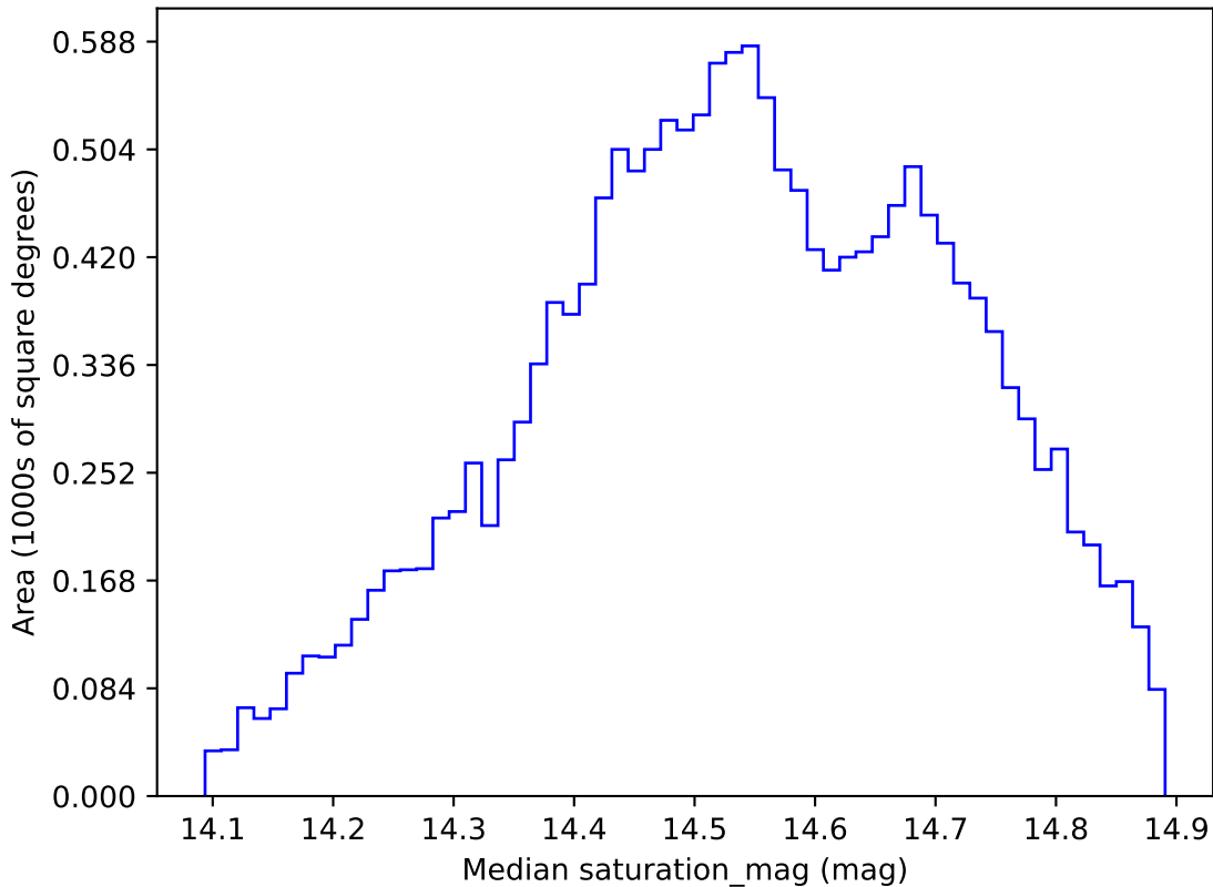
too_elab_r8_d2_griz_v3.4_10yrs WFD i band: Median saturation_mag
